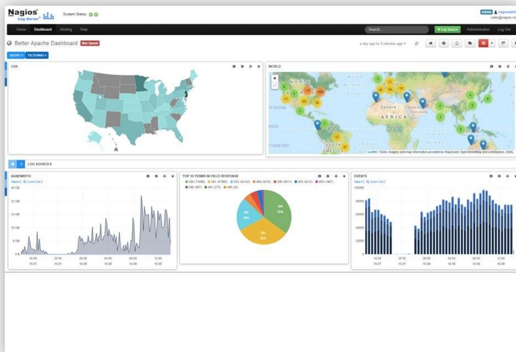
Figura 2 – Dashboard
